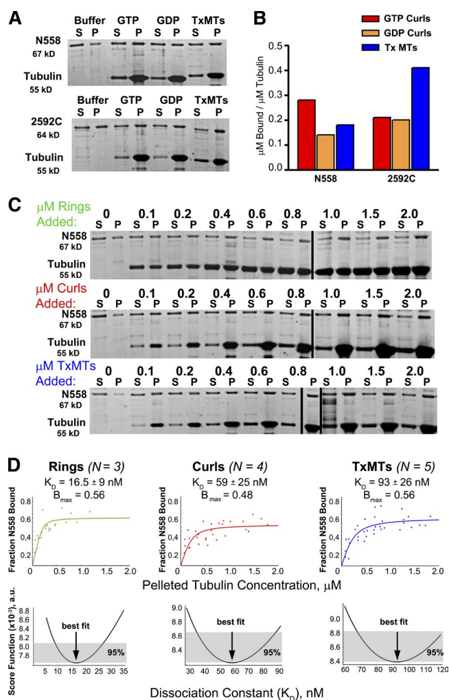
Figure 5. An N-terminal fragment of CENP-F binds better to curls than MTs, whereas a C-terminal segment does the opposite. (A) 0.2 \mu\text{M} N558 or 0.4 \mu\text{M} 2592C were mixed with buffer alone or with buffer including 0.4 \mu\text{M} tubulin assembled as GTP curls, GDP curls, or Tx-MTs, and then incubated and centrifuged as described in Materials and methods. Gels of supernatant and pellet fractions were stained with SYPRO Ruby (Molecular Probes). (B) Bound protein was measured by densitometry of the pellet fractions. The fraction of protein that pelleted nonspecifically in the buffer-only lane was subtracted from the values measured for each experiment. The amounts shown are from a single representative experiment out of four repeats for N558 and two repeats for 2592C. (C) 0.2 \mu\text{M} N558 was mixed with various concentrations of tubulin added as rings, curls, or Tx-MTs, and then incubated, centrifuged, and analyzed by gel electrophoresis and densitometry, as described in Materials and methods. (D) Protein amounts in each lane of three to five experiments, as in C, were quantified as in Materials and methods and the results were plotted. The data were fit with a quadratic model for protein binding by the method of least squares. Normalized score functions for goodness of each fit are shown in the bottom row. A value of 0 for this function would imply a perfect fit.
