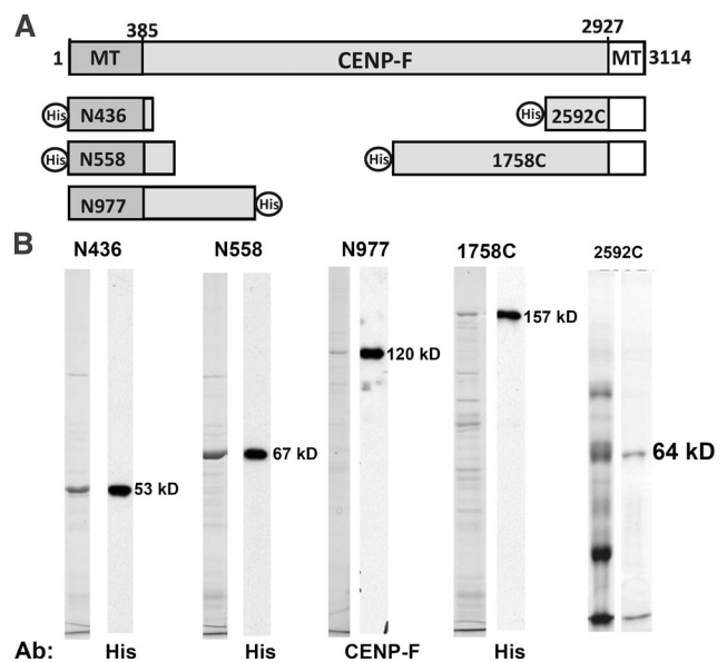
Figure 4. Fragments of CENP-F as expressed from cDNAs. N436, N558, 1758C, and 2592C were expressed in bacteria and N977 was expressed in SF9 cells, as described in Materials and methods. (A) The relationships between these pieces and the entire coding sequence of CENP-F. (B) For N436, N558, N977, and 1758C Coomassie-stained electrophoresis gels of the partially purified fragments and adjacent immunoblots with anti-penta-his (QIAGEN) or anti-CENP-F, confirming that the proteins isolated are the ones expressed. For 2592C, the peak fractions from Ni 2+ -NTA (left) and from a HiTrap SP column (right) stained with Coomassie.
